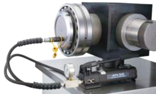
Hydraulic dismounting
